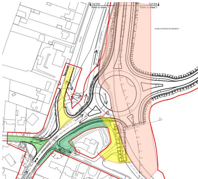
Figure 1 – Current Layout
