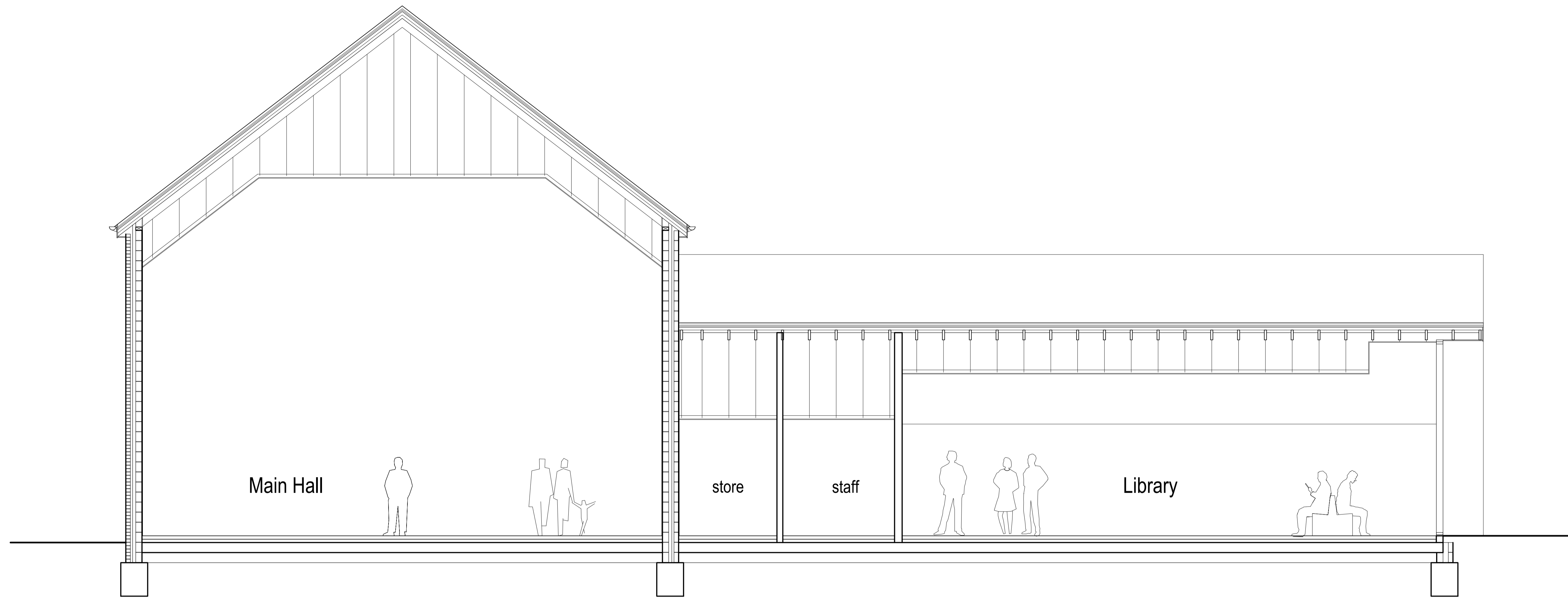
Section B-B
