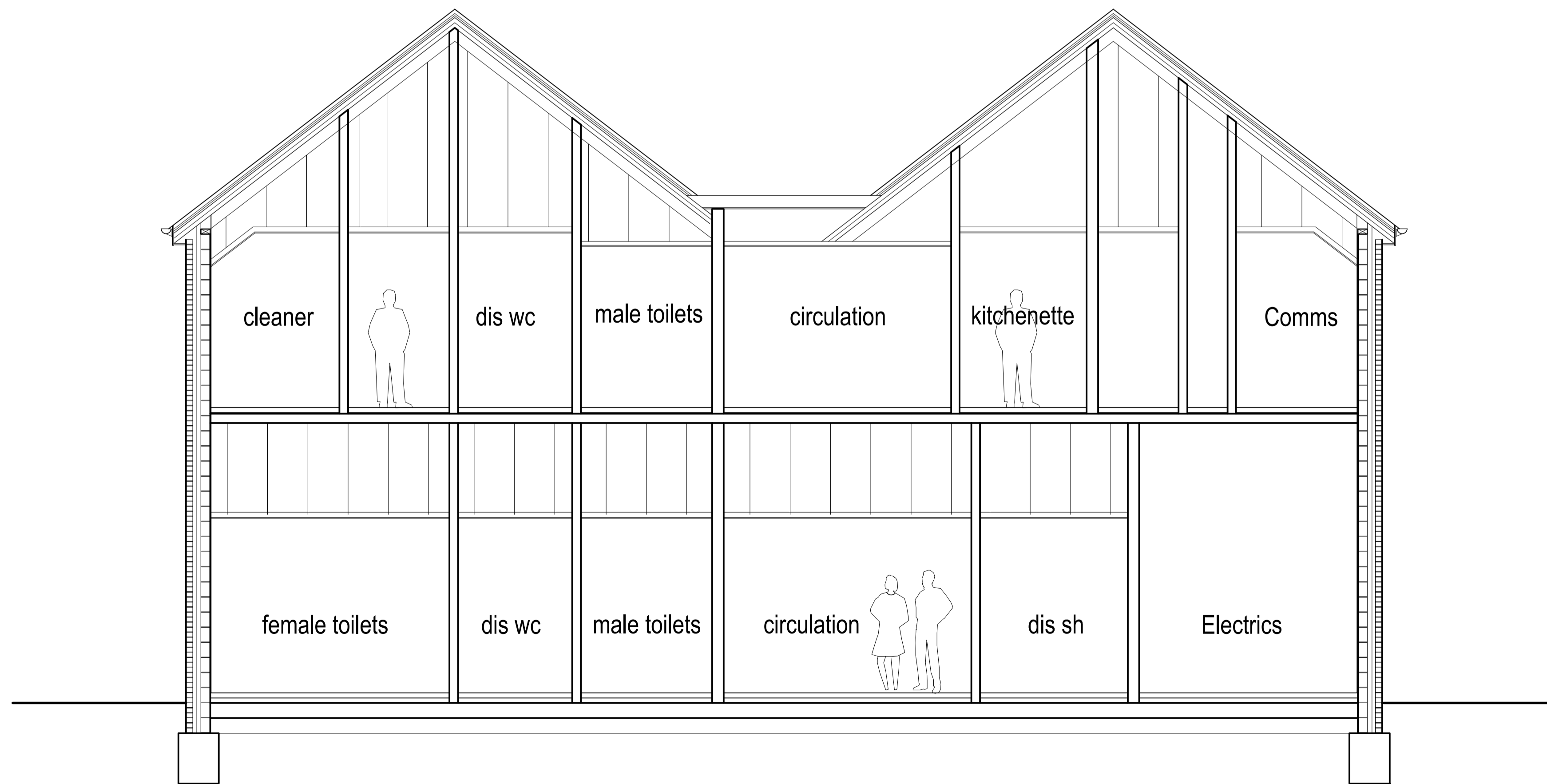
Section C-C
